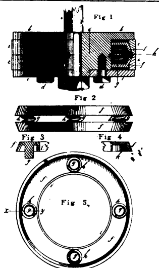
35011 Stafford's Piston.
