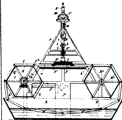
27433 Prichard's Surfacing Machine.
