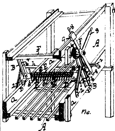
27437 Briggs' Apparatus for Planing Ice.
