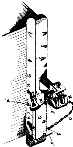
27432 Harrington's Car Coupler.
