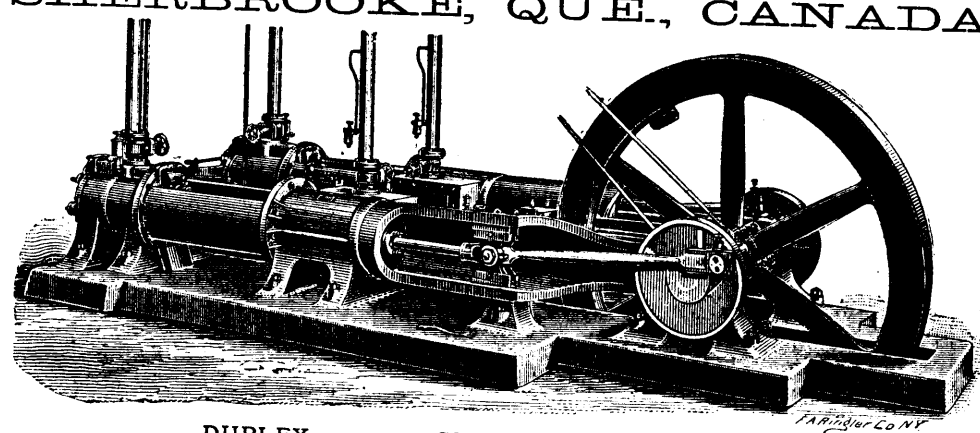
DUPLEX 14 x 22 STEAM AIR COMPRESSOR.
