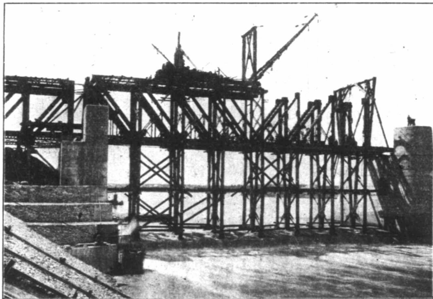
10 Erection of Steel Work, St. Andrews Locks, Red River
