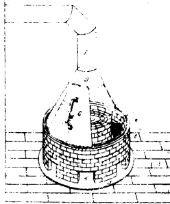
12553 Bredannaz's Kiln for Heating Wheel Tires.
