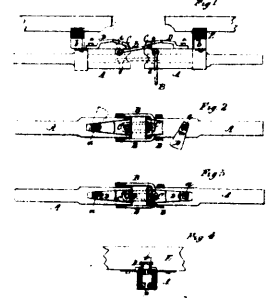
12554 Murray's Improvements in Car-couplings.
