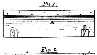
12563 Craig's Improvements on Stave Knives.
