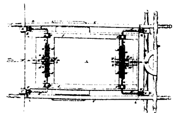
12566 Rice's Improvements on Vehicle Springs.
