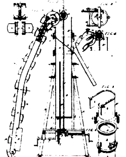
12557 Smith's Improvements on Elevating Apparatus.
