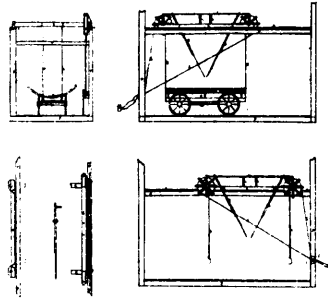
12562 Sargent's Load-lifter.
