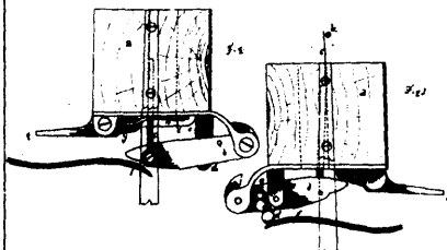
6630 Jones' Machine for Opening and Closing Blinds and Shutters.
