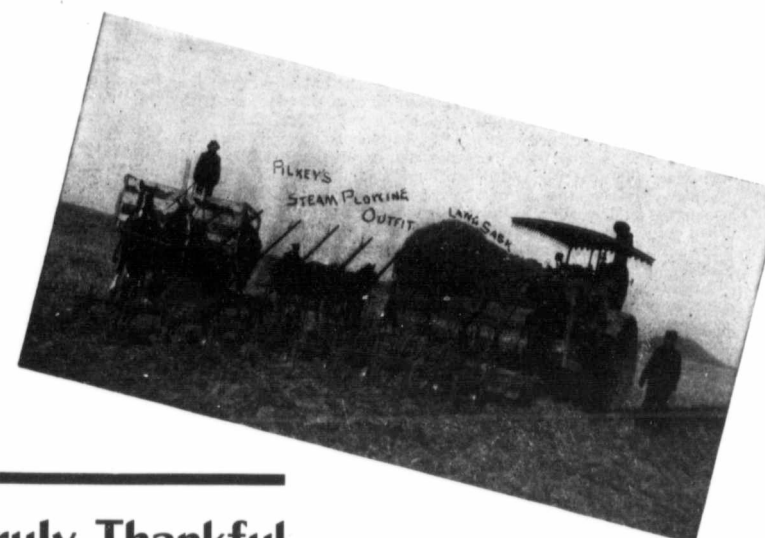
Gaar-Scott 33 h.p. Canadian Special plowing with twelve 14-inch bottoms. Burns straw only and has plenty of power.
