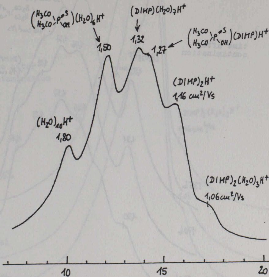
Fig. 10: IMS spectrum recorded at measurement point 5, approx. 45 ppb DIMP were added into the gas stream sampled from the joint
