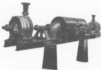
Two Worthington 3 stage Turbines and McCormick Water Wheels, built for Port Arthur, Ontario, Water Works. Combined capacity 1440 gallons per minute against 350 head.
