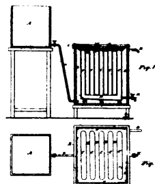
8389 Bowen's Improvements on Milk Coolers.
