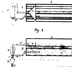
8381 Fordon's Improvement in Steam Boiler Cleaners.
