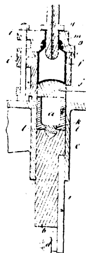
33904 Ryland's Machine for Forming Bottles.
