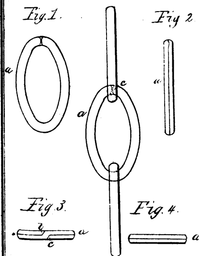
Fisher's Split Ring.
