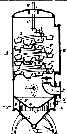
Ward's Feed Water Heater and Purifier.
