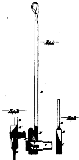
18890 Wood's Knitting Machine Needle.
