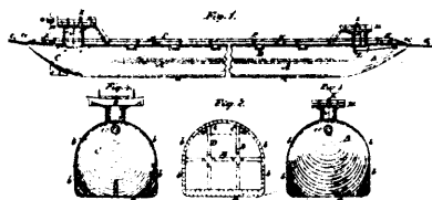
14644 McDougall's Improvements on Tow Boats.
