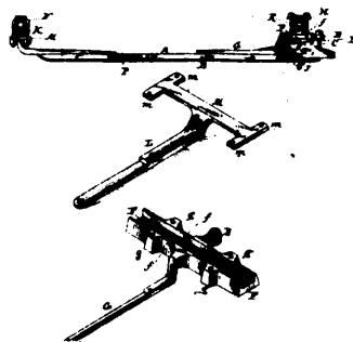
14656 Herbrand's Improvements in Running Gears for Vehicles.
