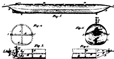
14950 McDougall's Improvements in Tow Boats.
