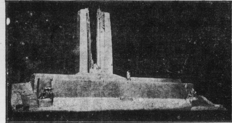
Mr. Walter S. Allward's design for a memorial on Hill 62, overlooking the Ypres Salient. This memorial was accepted by the Canadian Battlefields Memorial Commission. It is approximately 225 feet long and between 125 and 140 feet high at its highest point.
