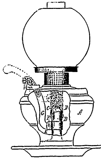
28352 Rhind's Wick Lifting Device.
