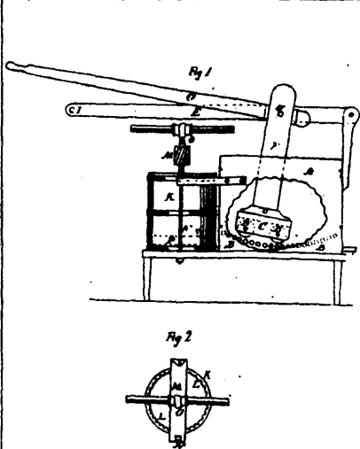
18219 Ketchum's Improvements in Button Fasteners.
