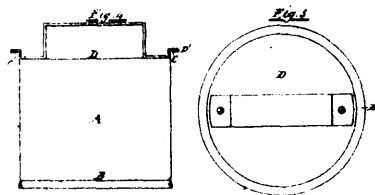
13088 Austin's Improvements on Metal Cans.
