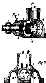
13087 Hancock's Improvements on Valves.
