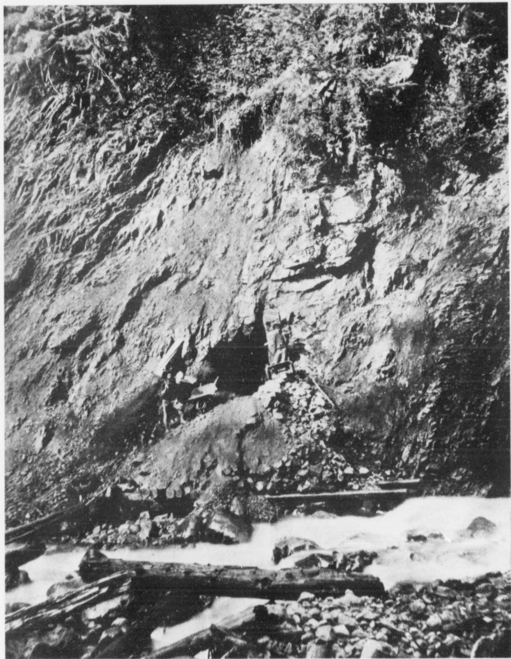
UPPER TUNNEL, ROOSEVELT CLAIM, SHOWING QUARTZ VEIN IN FACE OF BANK.
