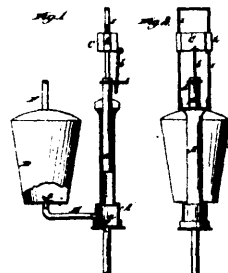
11764 Hoover & Van Sickle's Improvements on Pumps.
