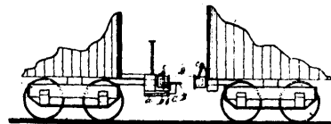
11761 Laroque's Improvements in Car-couplings.
