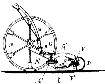
10826 Garvin's Improvements in Mowing Machines.
