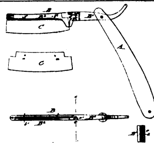
5240 Erdmansk's Improvements on Razors.
