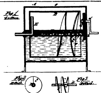
5243 Reed's Air Blower for Carburettors.
