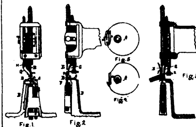
5246 Ballou's Boot and Shoe Wax Thread Sewing Mechanism.
