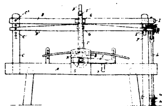
14953 McCloskey's Spoke Guide and Gauge.
