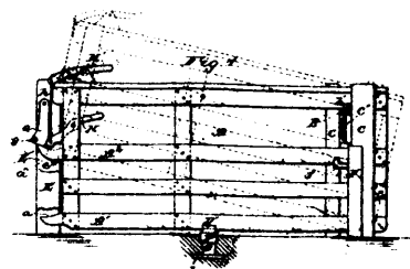
14956 Sherwin's Improvements on Gates.
