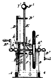
14949 Mershen's Improvements on Rock Drills.
