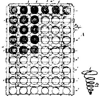
14951 Whitaker's Improvements on Spring Beds.
