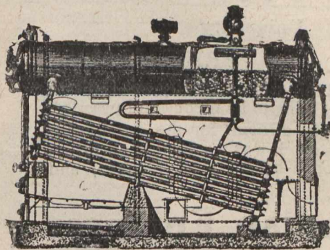
'B. &amp; W.' Boiler Fitted with Superheater.
