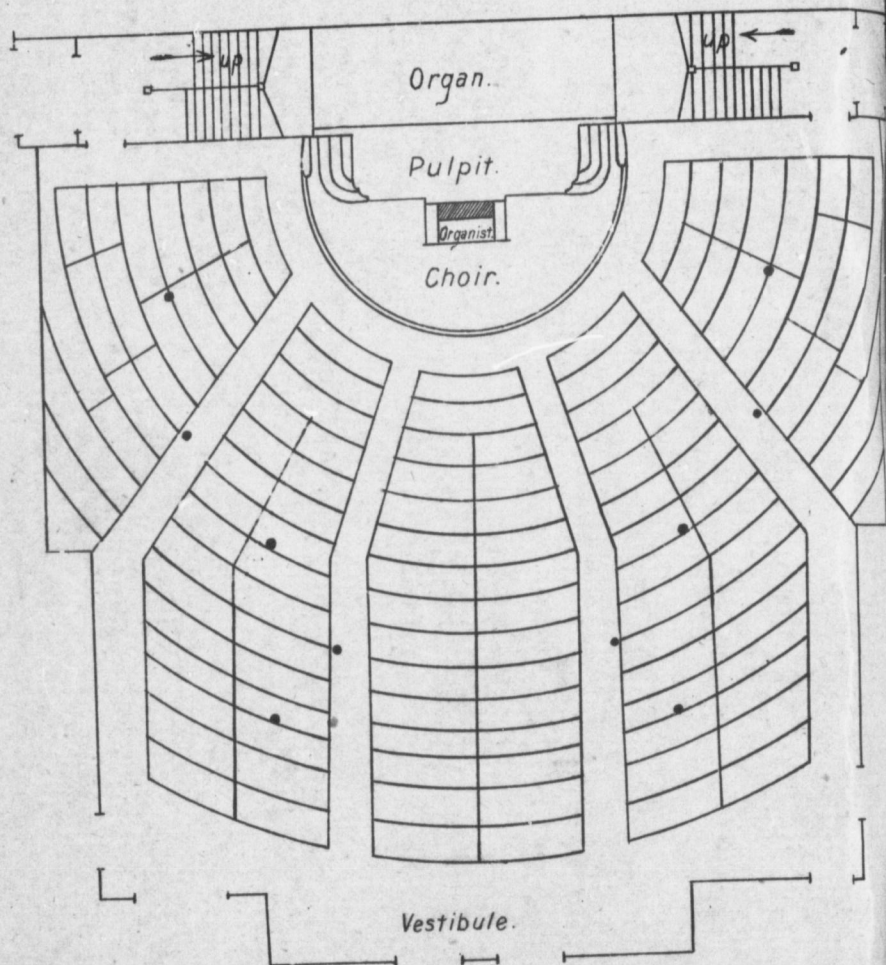
PLAN OF GROUND FLOOR
