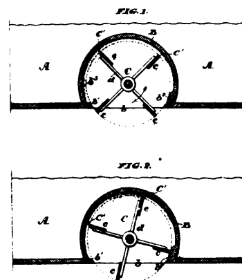
38124 Wigmore's Ship Propeller.
