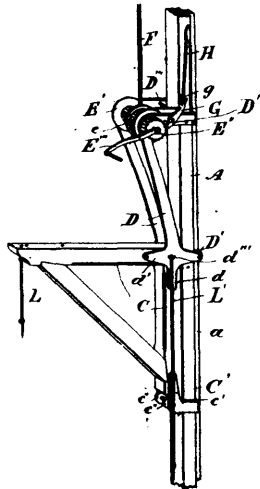
35539 Downie's Scaffold.
