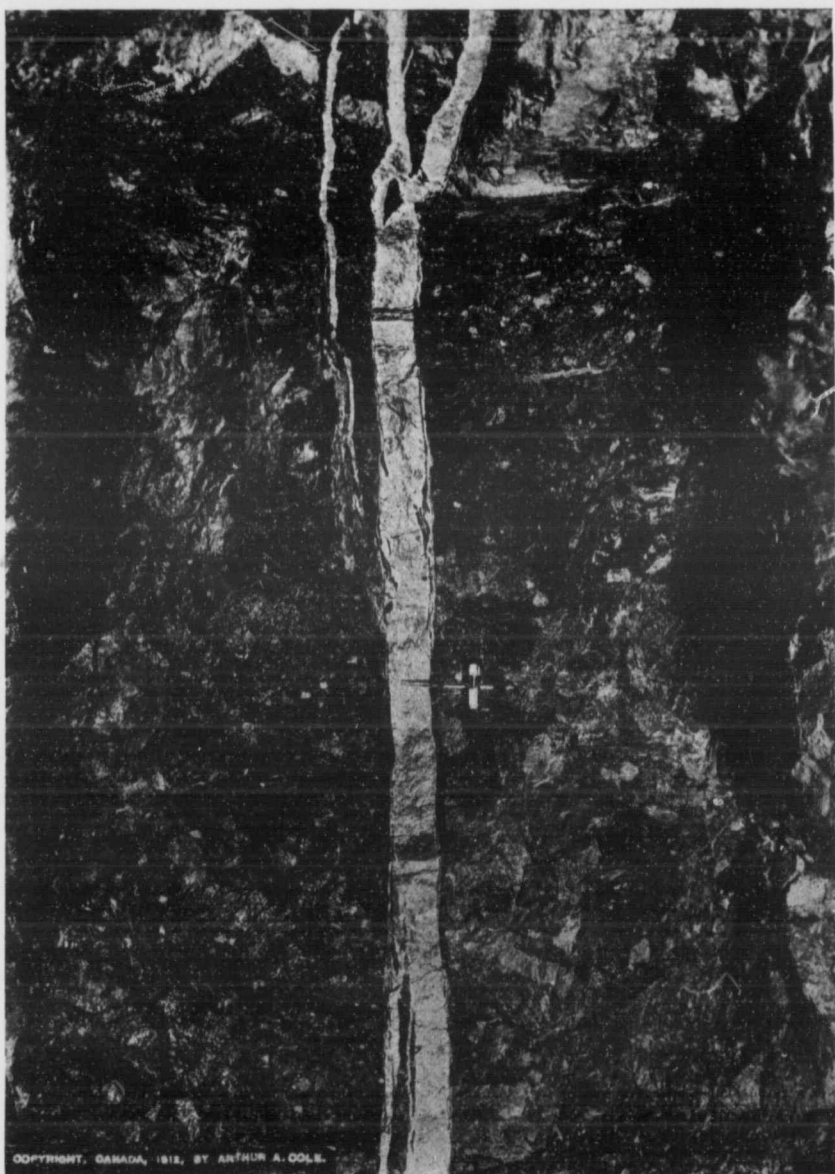
A High Grade Silver Vein in a Cobalt Silver Mine. Cobalt, Ontario, Canada.
