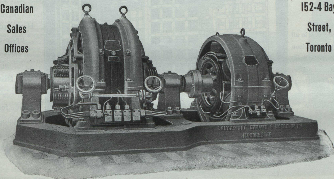
Standard Patent Automatic Reversible Booster 2,000 Ampere Size
