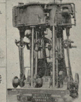
15 and 30 x 20 FOR. AND AFT. COMPOUND MARINE ENGINE WITH STEAM REVERSE
