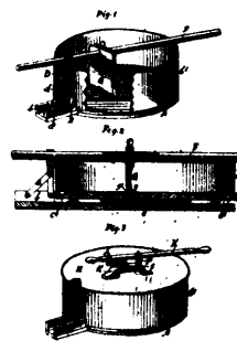
9826 Rideout's Combined Churn and Butter Worker.
