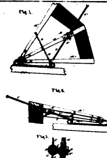
9835 Hayes's Improvements on Vehicle Tops.
