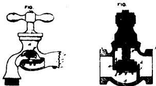
9827 Little &amp; Smart's Improvements on Valves.
