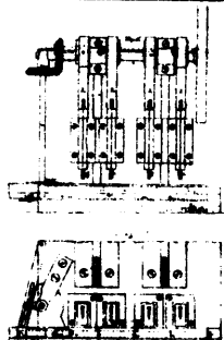
No. 1802. Owyll's Machine for Punching Horse-Shoe Nail Blanks.
