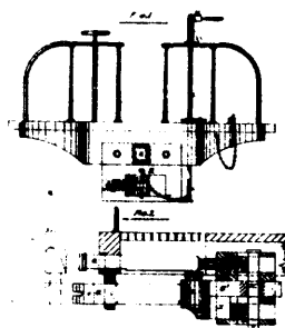
No. 1799. Willson's Car-Coupler with Compressed double or single Buffer Combined.
