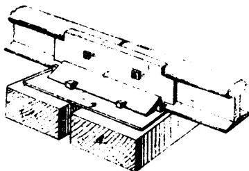
No. 1795. Williams' Ball-Joint.
