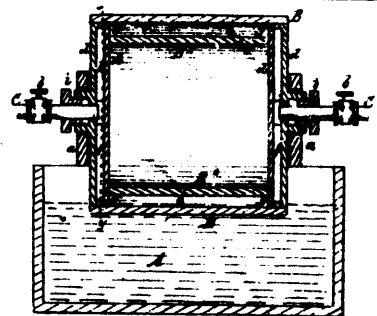
No. 1797. Gilson's Apparatus for manufacturing Salt.
