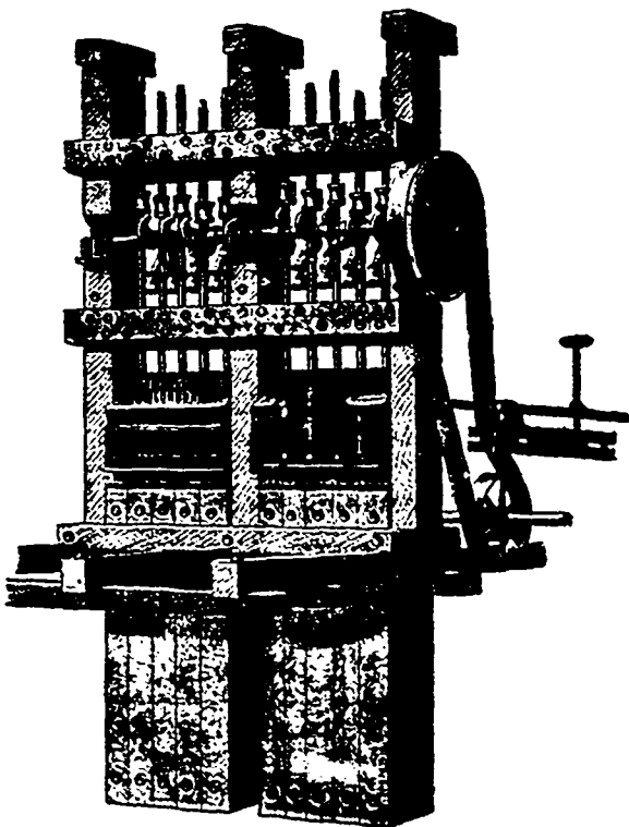
Stamp Mills, Huntington Mills, Ore Crushers Concentrators, etc.
