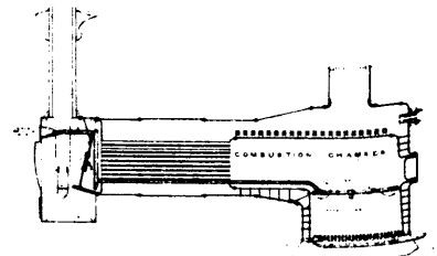
9665 Lett's Device for Arresting Sparks and Burning the Smoke for Locomotives.
