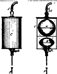
7128 Robertson's Tank for Supplying Water to Closets.
