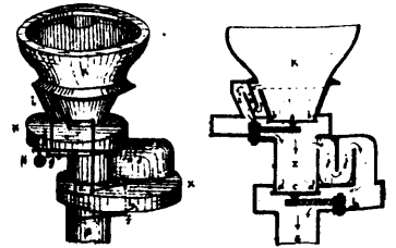
7127 Robertson's Method of Constructing Water Closets.
