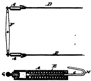
7131 Berry's Spring Draft Attachment to Traces.
