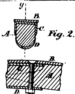
7134 Bowerman's Improved Felly Joints.
