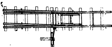
7124 Bagnall & Hall's Improvements in Railway Switches.
