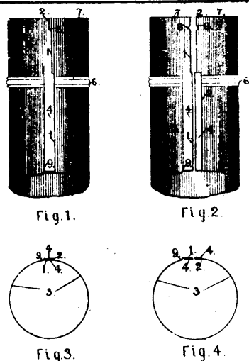
36762 Curtis' Pipe Wrench.
