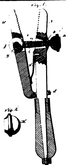
36762 Curtis' Pipe Wrench.
