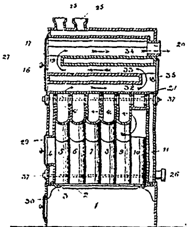
7878 Gate's Hot Water Boiler.
