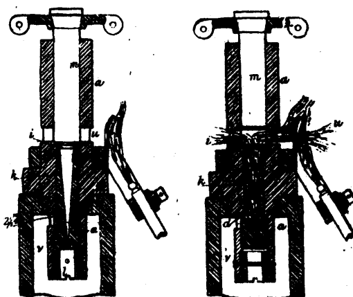
Figs. 5 and 6.—Igniting Arrangement.
