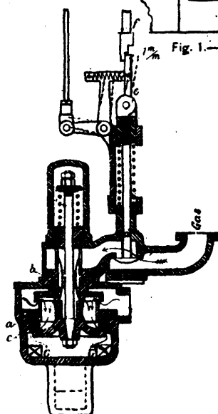
Fig. 4.—Mixing-Valve.
