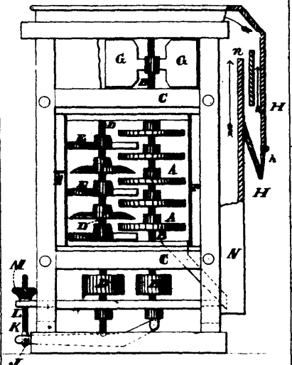
27508 Yates' Grain Scourer.
