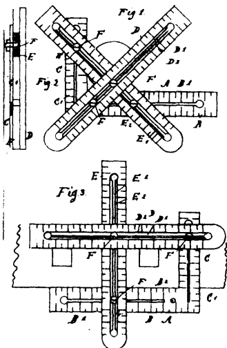
27512 Kliff's Measuring Instrument.
