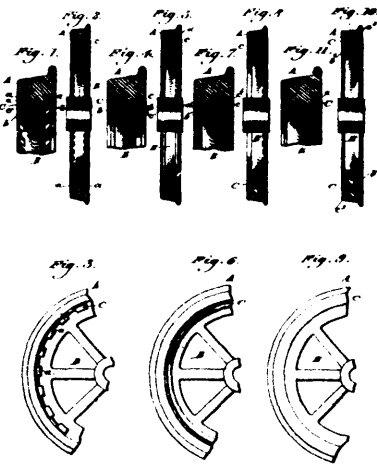
27509 Cloud's Locomotive and Car Wheel.
