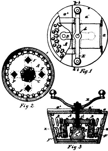
18557 Parisault's Washing Machine.
