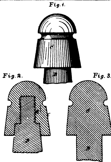
13561 Hildale's Telegraph Insulator.
