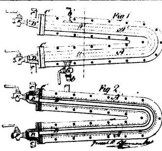
12409 Blumenberg's Improvements on Condensers.
