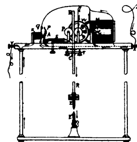
12407 Houston & Thomson's Improvement on Regulators for Electric Lamps.
