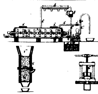
12411 Bell & Sloane's Process of Purifying Waxes, Resins, Gums and Fatty Matters.
