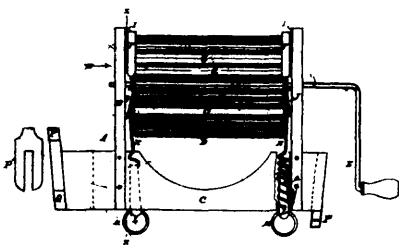
2512 Calkins' Washing Machine.
