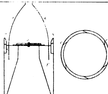
6858 Cochran's Improvement on Pumps.
