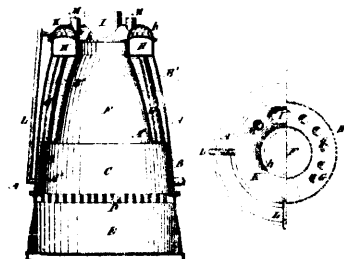
6853 Chanceloup's Improvements in Hot Water Furnaces.
