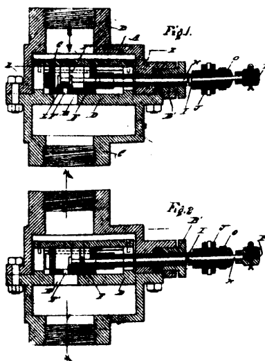
34537 Leslie's Throttle Valve.
