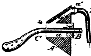
34530 Dooley's Lamp Bracket.
