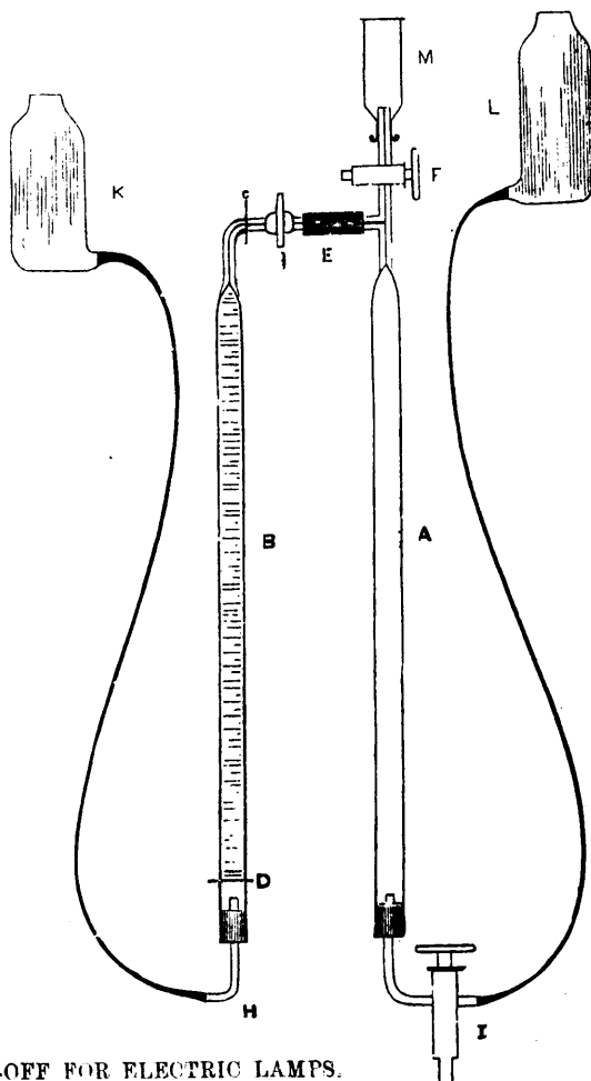
RAPIÉFF'S CUT-OFF FOR ELECTRIC LAMPS.
