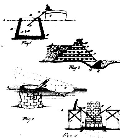
26490 Goodridge's Method of Laying Concrete Under Water.
