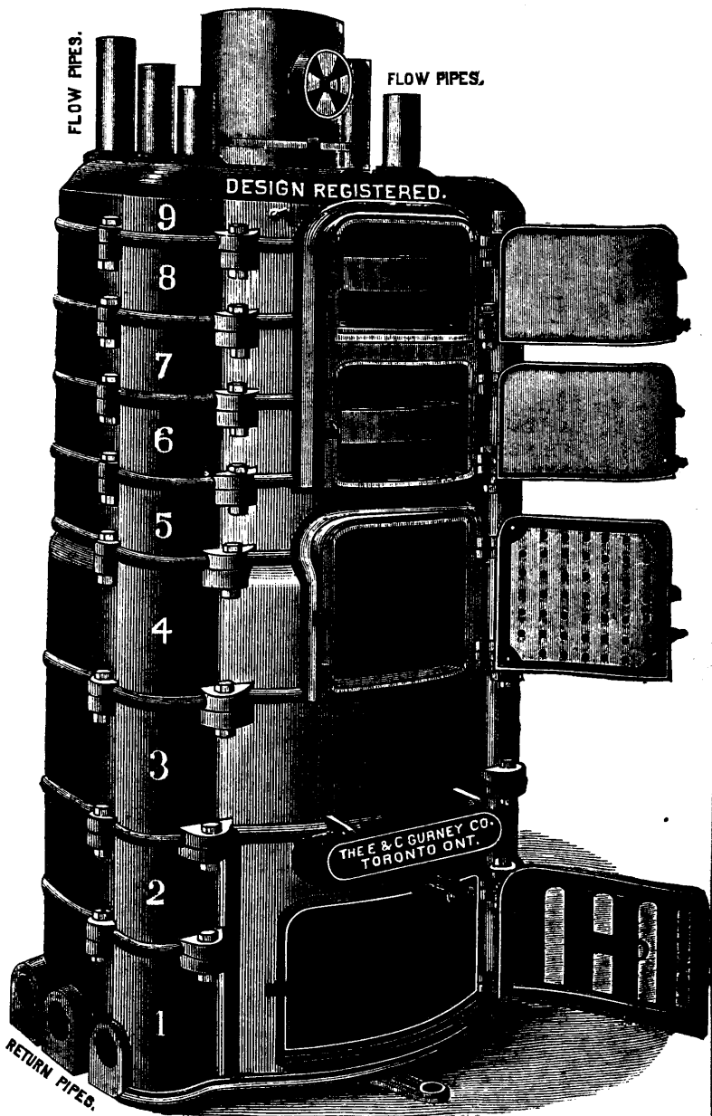
FRONT AND SIDE VIEW.
