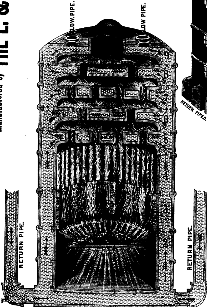
CONSTRUCTION AND CIRCULATION OF WATER AND HEAT.
