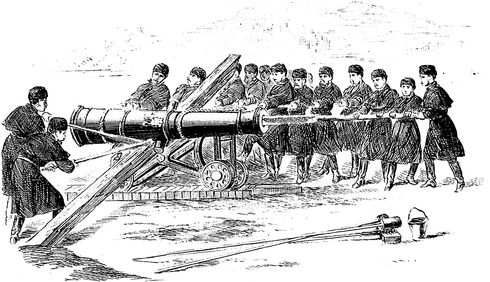
Mounting a 32 cwt. 32-pounder on an iron carriage by a single timber under the centre of gravity
