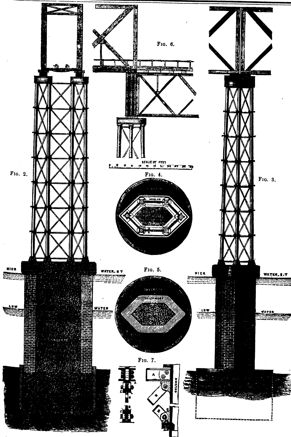
FIG. 2. SIDE ELEVATION. FIG. 3. END ELEVATION OF PIER. FIG. 4. PLAN OF PIER. FIG. 5. PLAN OF PIER MASONRY. FIG. 6. JUNCTION OF LARGE AND SMALL SPANS. FIG. 7. SECTION OF COLUMN JOINTS.
