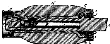
10592 MacKinnon's Improvements in Axle Boxes.
