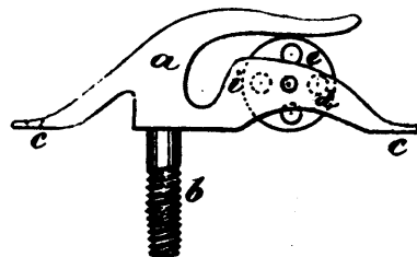
10590 Robinson's Improvements on Holdbacks for Vehicles.
