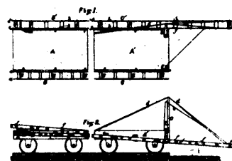
10593 Moore's Apparatus for Unloading Railway Rail and Ties.
