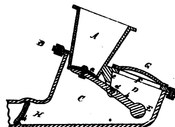
10600 Haynes, Fitts &amp; Caled's Improvements on Sewer Traps.
